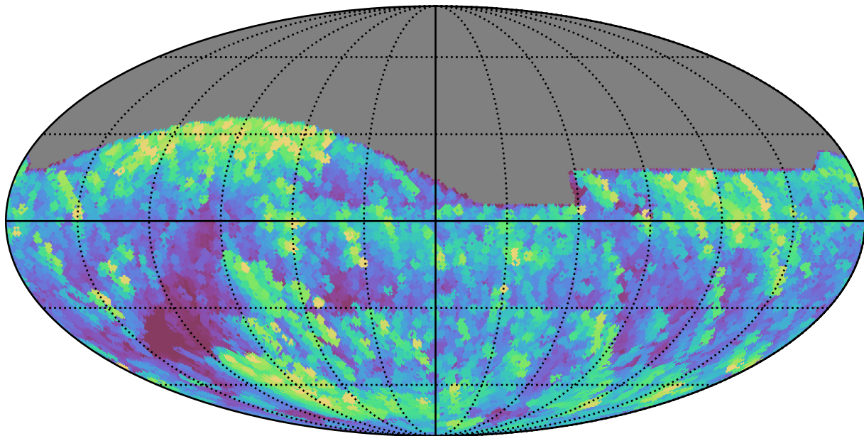
baseline_v3.0_10yrs All sky r band: Max airmass
