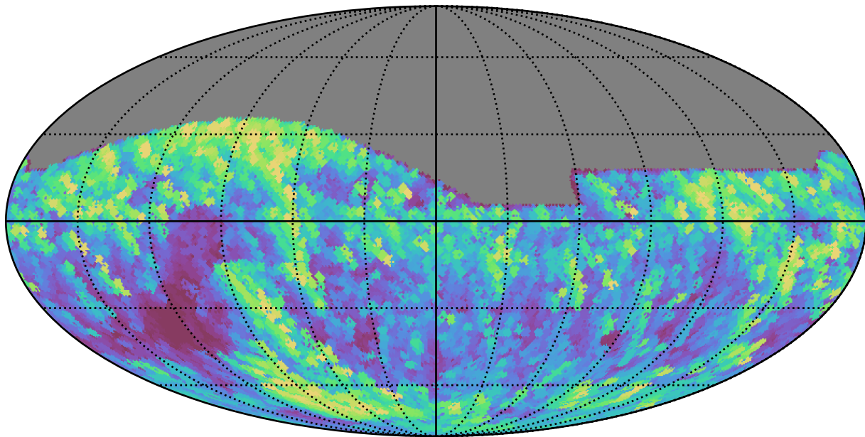
baseline_v3.0_10yrs All sky i band: Max airmass
