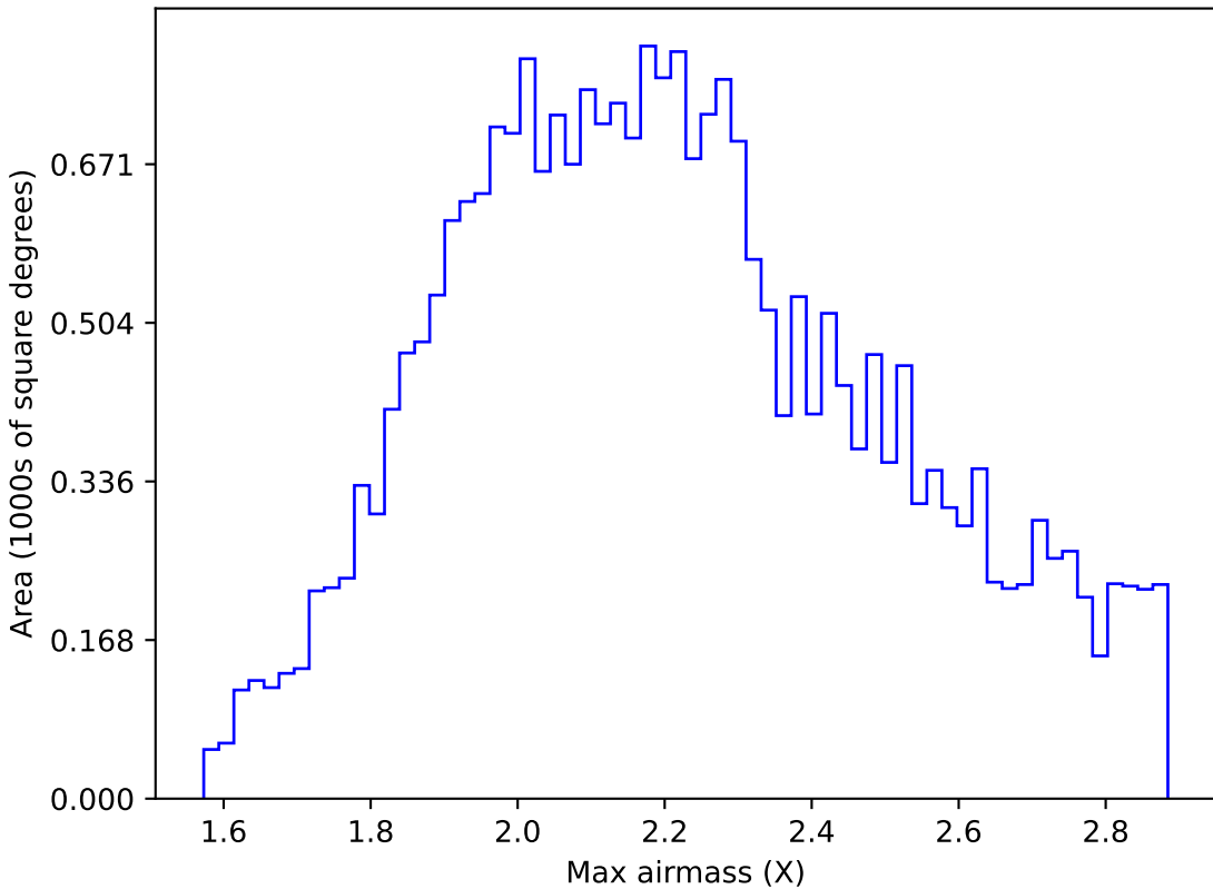
baseline_v3.0_10yrs All sky i band: Max airmass
