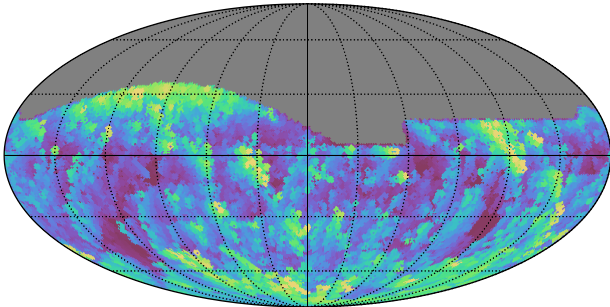
baseline_v3.0_10yrs All sky g band: Max airmass
