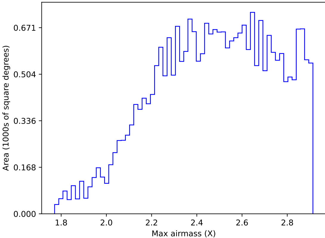
baseline_v3.0_10yrs All sky all bands: Max airmass
