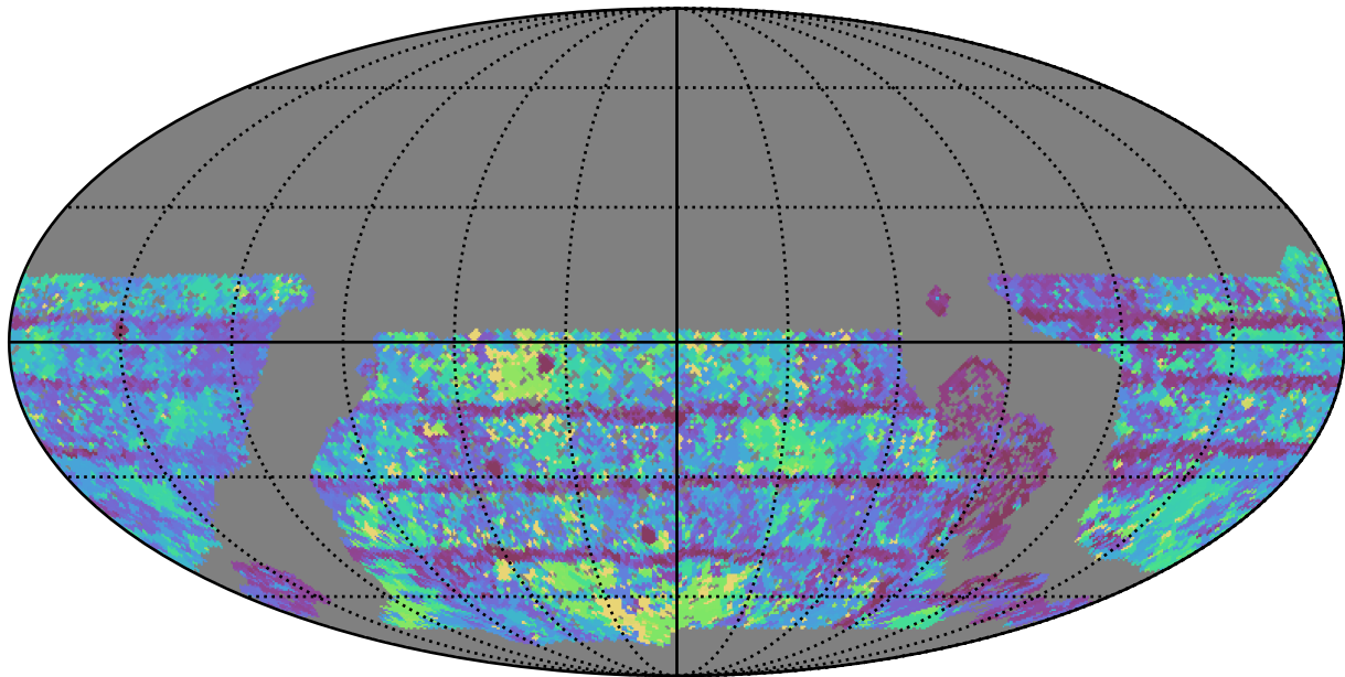
baseline_v3.0_10yrs WFD z band: Max Inter-Night Gap
