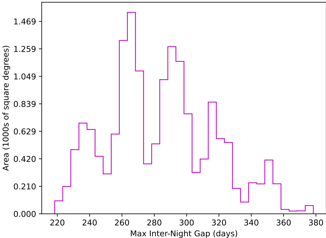
baseline_v3.0_10yrs WFD z band: Max Inter-Night Gap
