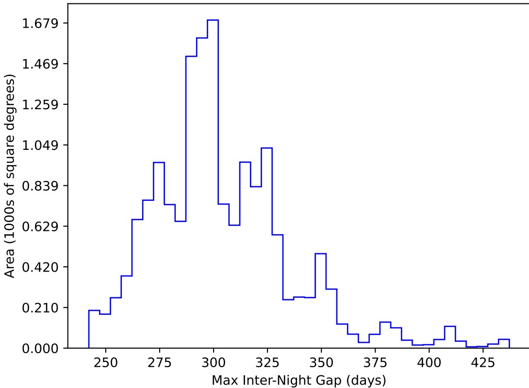
baseline_v3.0_10yrs WFD y band: Max Inter-Night Gap
