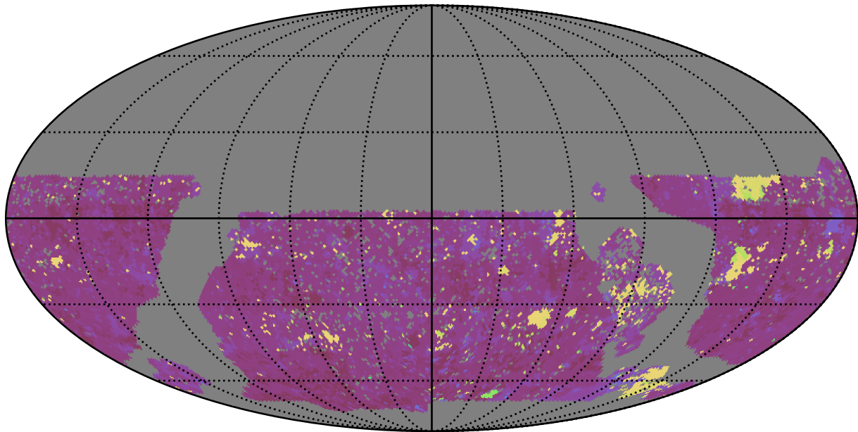
baseline_v3.0_10yrs WFD u band: Max Inter-Night Gap
