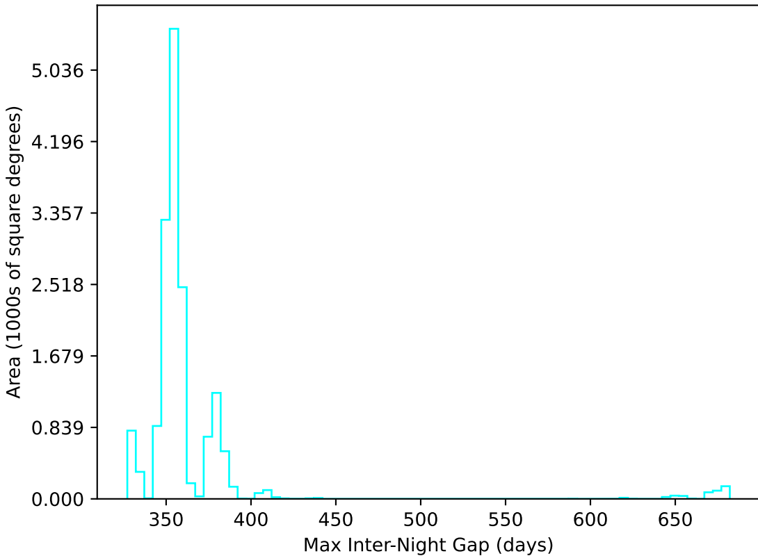
baseline_v3.0_10yrs WFD u band: Max Inter-Night Gap
