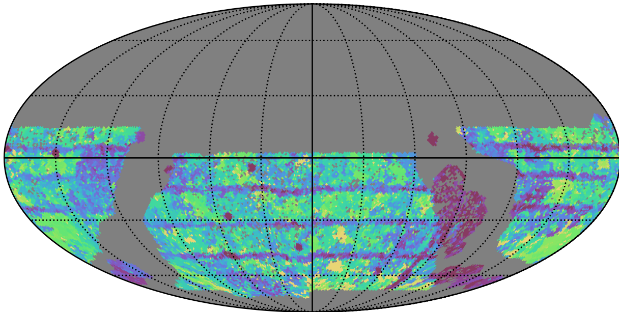
baseline_v3.0_10yrs WFD r band: Max Inter-Night Gap
