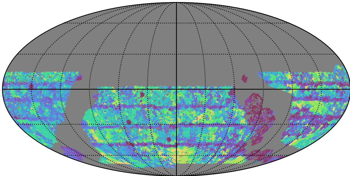
baseline_v3.0_10yrs WFD i band: Max Inter-Night Gap
