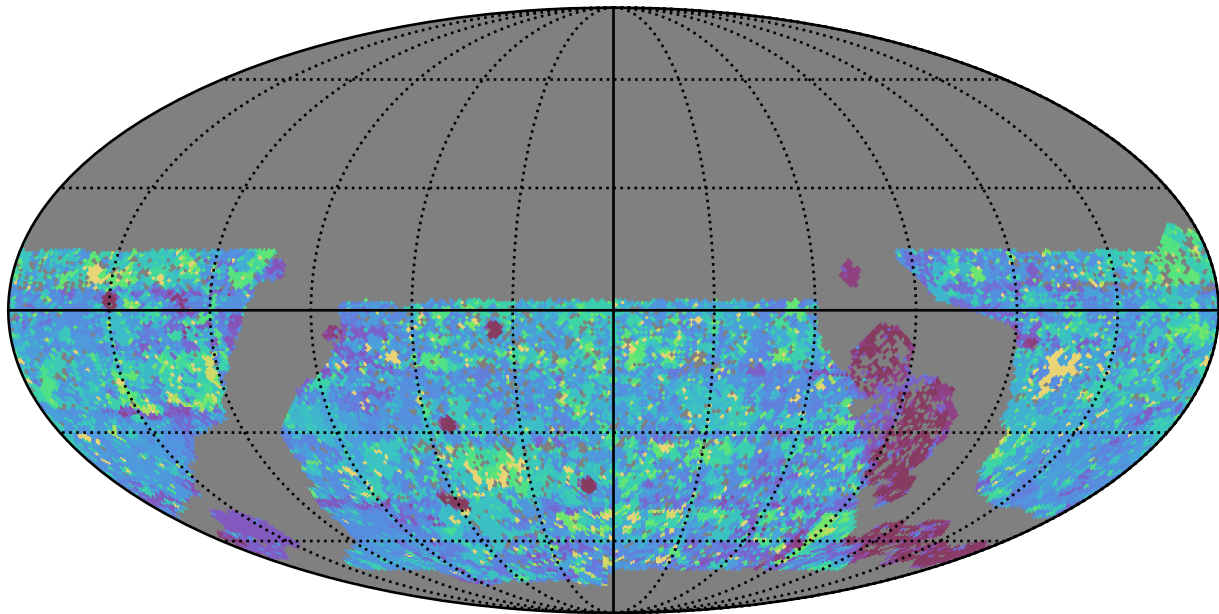
baseline_v3.0_10yrs WFD g band: Max Inter-Night Gap
