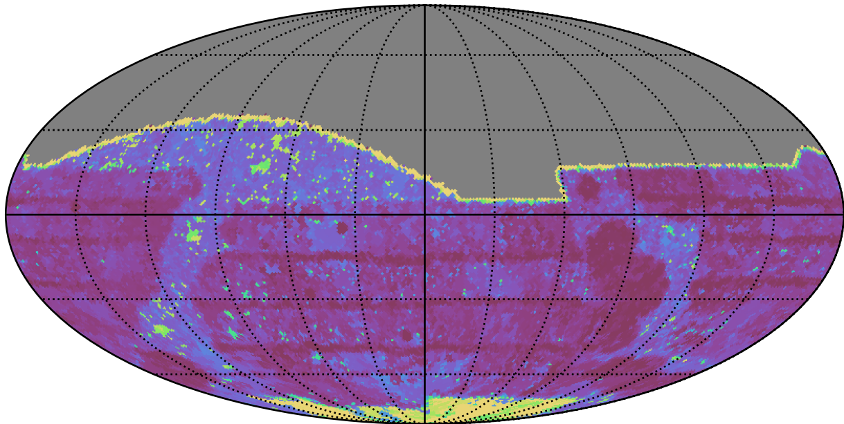
baseline_v3.0_10yrs All sky z band: Max Inter-Night Gap
