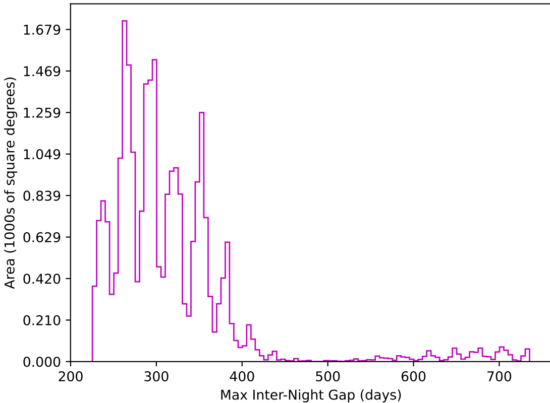
baseline_v3.0_10yrs All sky z band: Max Inter-Night Gap
