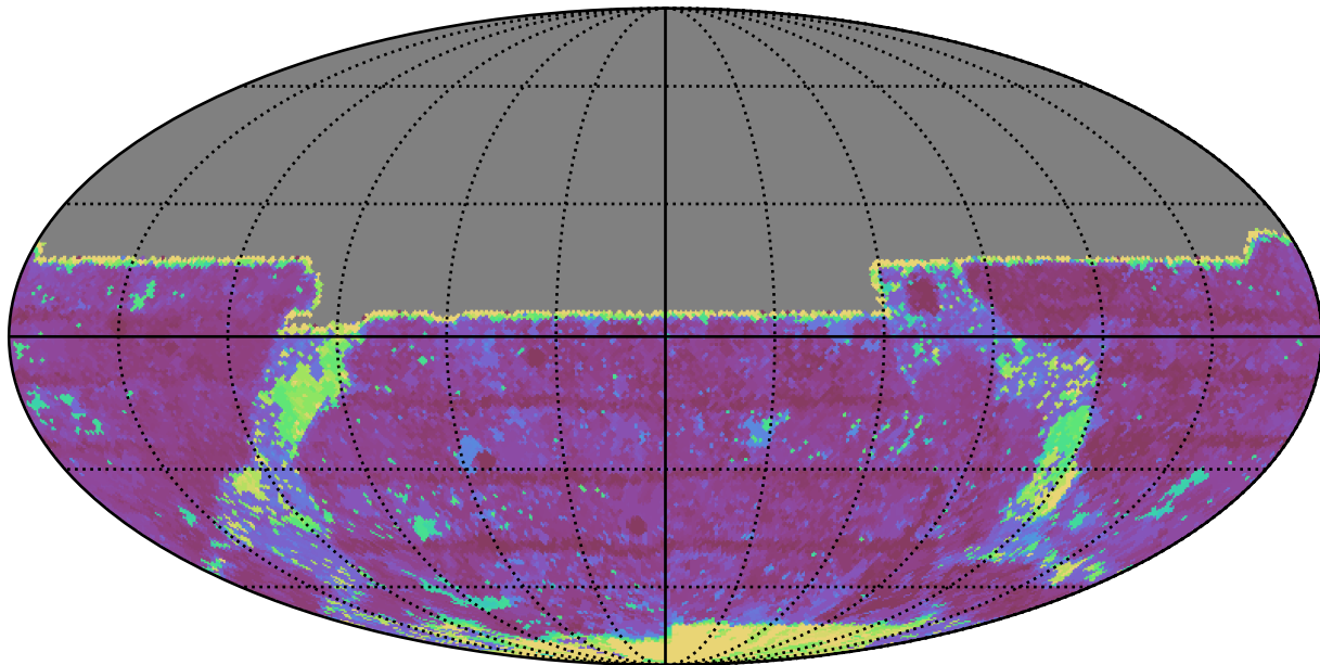
baseline_v3.0_10yrs All sky y band: Max Inter-Night Gap
