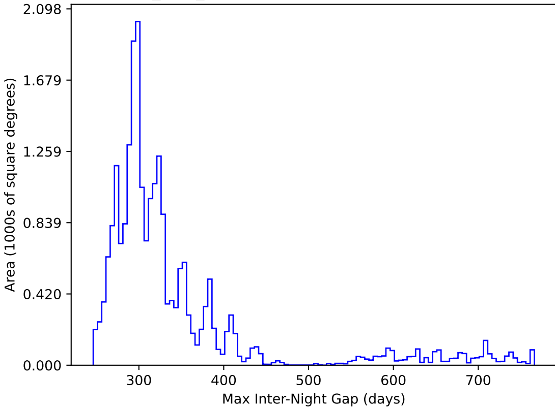
baseline_v3.0_10yrs All sky y band: Max Inter-Night Gap
