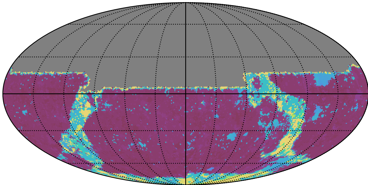
baseline_v3.0_10yrs All sky u band: Max Inter-Night Gap
