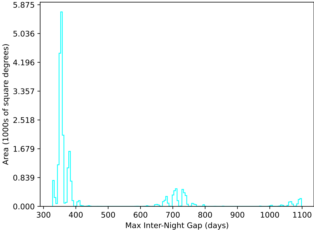
baseline_v3.0_10yrs All sky u band: Max Inter-Night Gap
