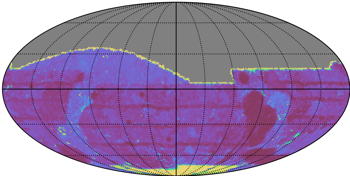
baseline_v3.0_10yrs All sky r band: Max Inter-Night Gap
