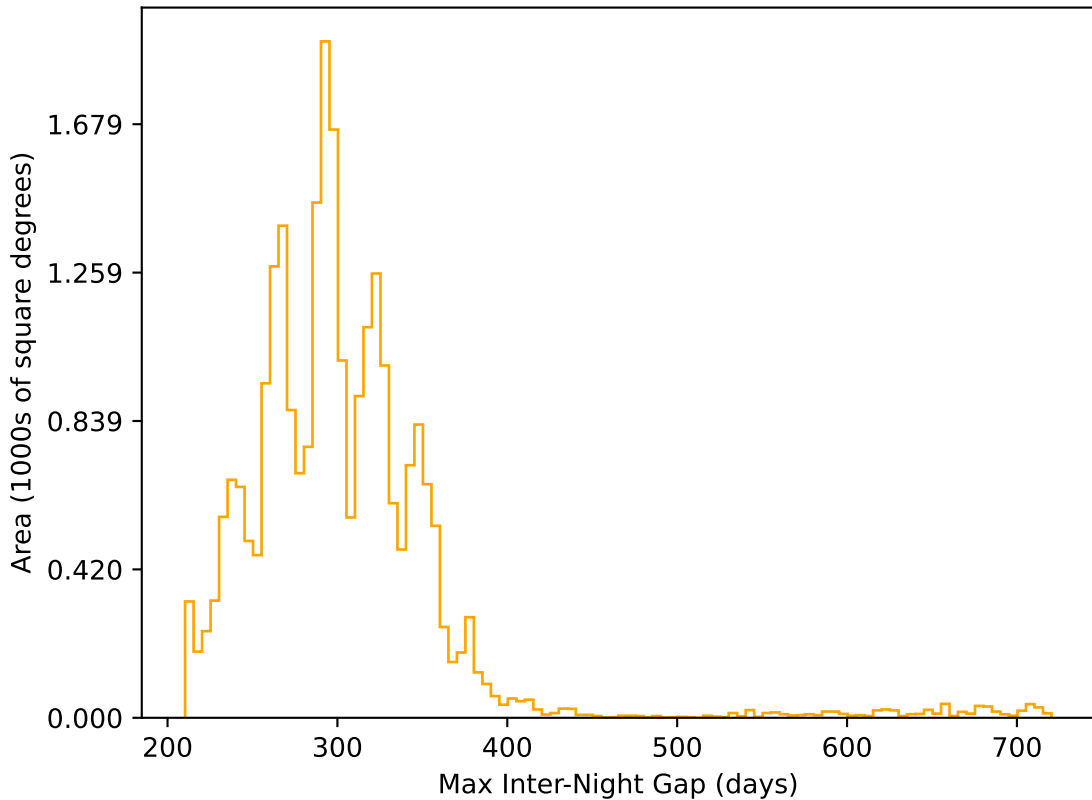
baseline_v3.0_10yrs All sky r band: Max Inter-Night Gap
