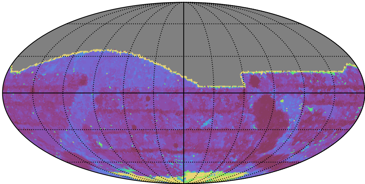
baseline_v3.0_10yrs All sky i band: Max Inter-Night Gap
