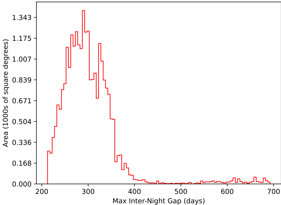
baseline_v3.0_10yrs All sky i band: Max Inter-Night Gap
