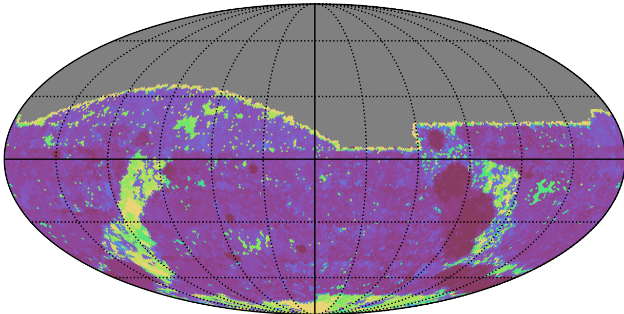
baseline_v3.0_10yrs All sky g band: Max Inter-Night Gap
