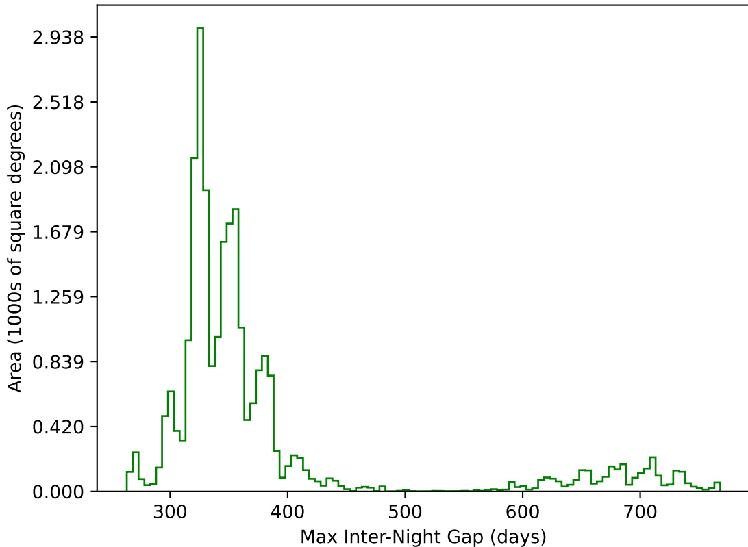
baseline_v3.0_10yrs All sky g band: Max Inter-Night Gap
