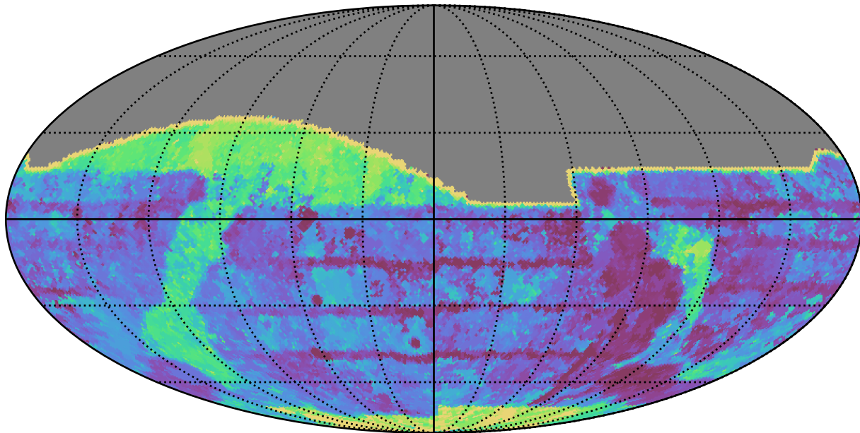
baseline_v3.0_10yrs All sky all bands: Max Inter-Night Gap
