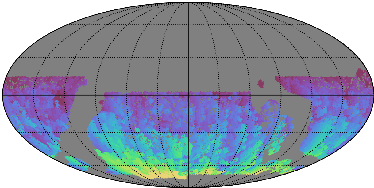
baseline_v3.0_10yrs WFD z band: Max HA
