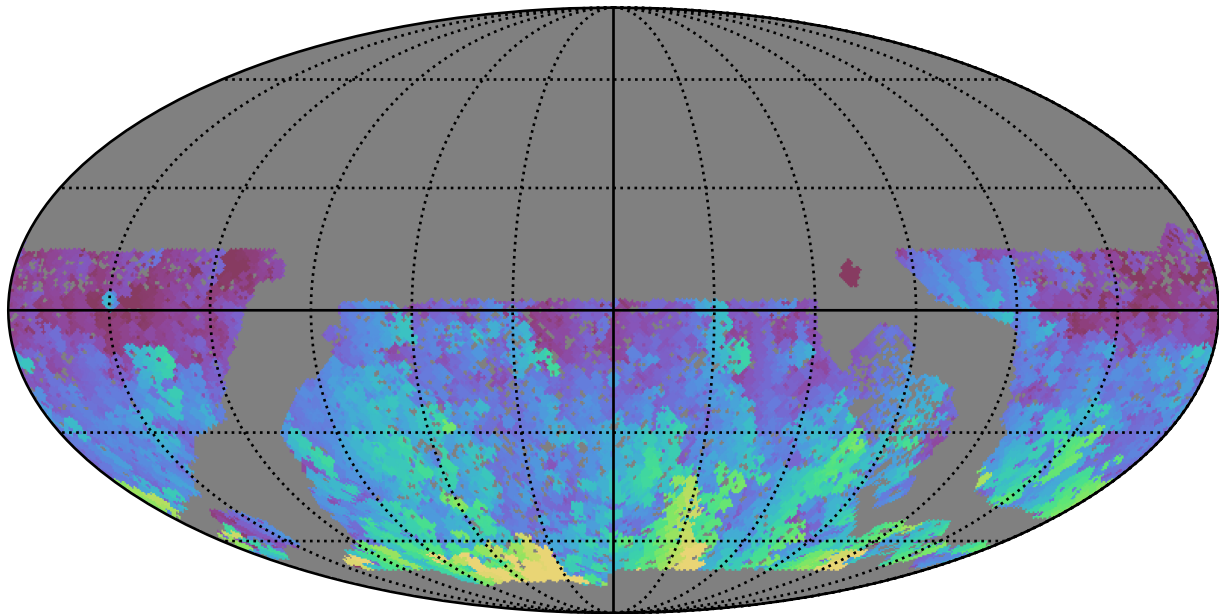
baseline_v3.0_10yrs WFD u band: Max HA
