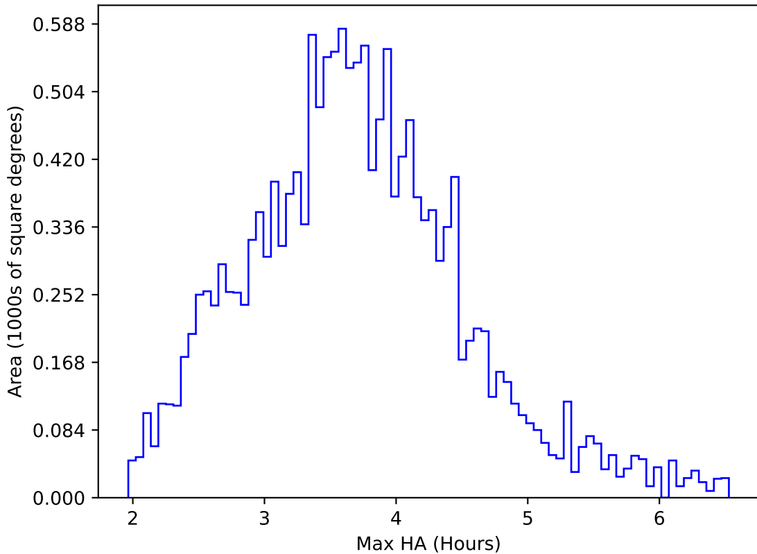
baseline_v3.0_10yrs WFD u band: Max HA
