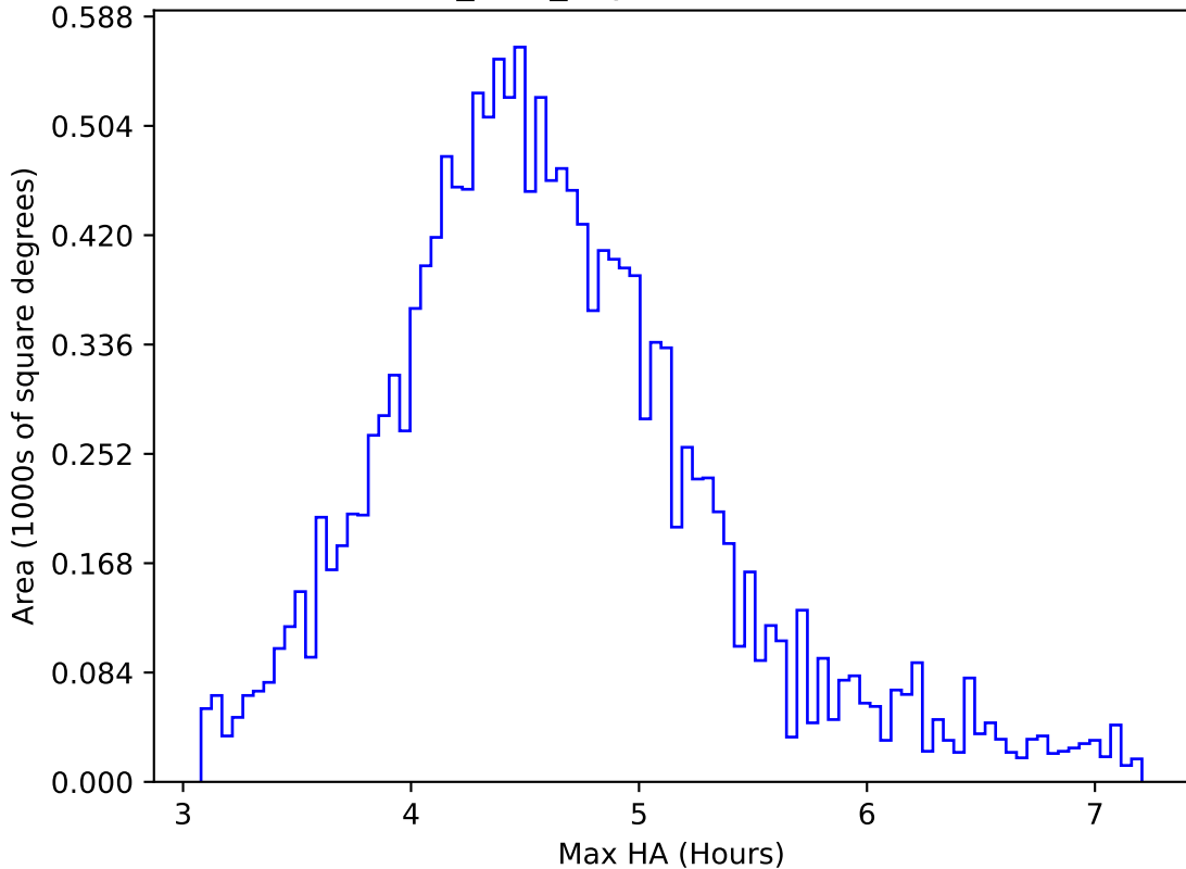
baseline_v3.0_10yrs WFD i band: Max HA
