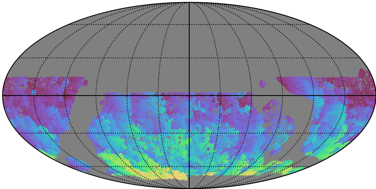
baseline_v3.0_10yrs WFD g band: Max HA
