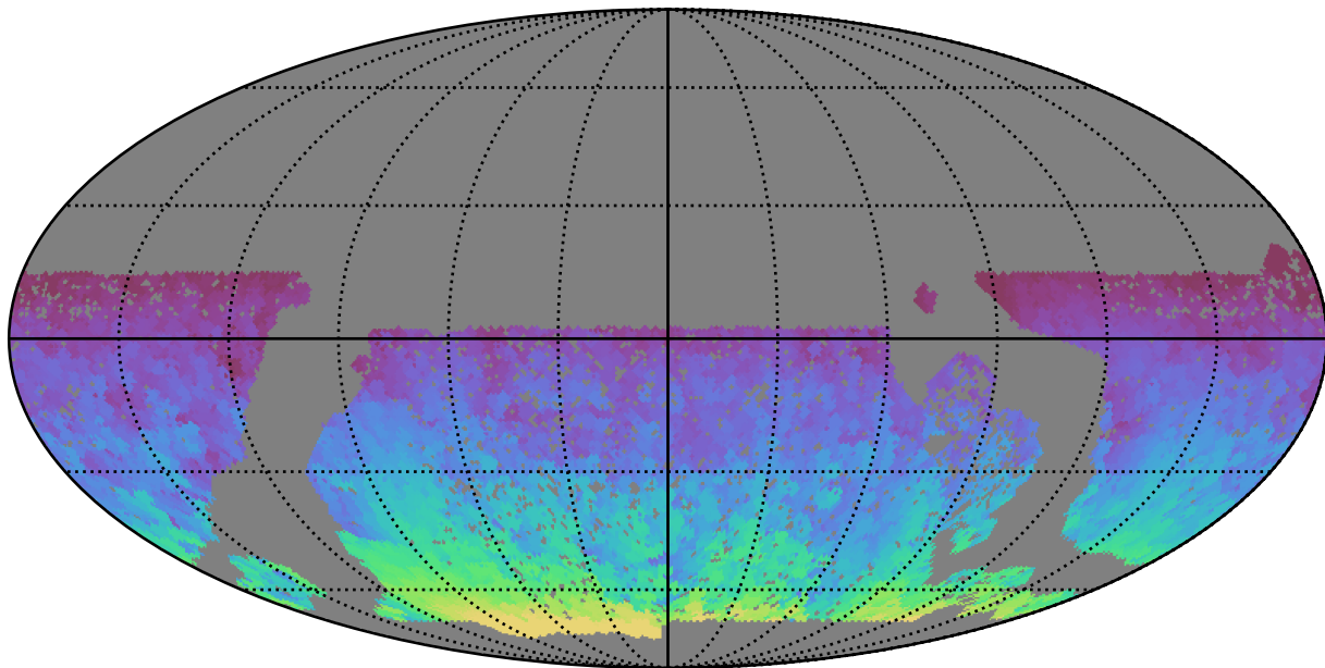
baseline_v3.0_10yrs WFD all bands: Max HA
