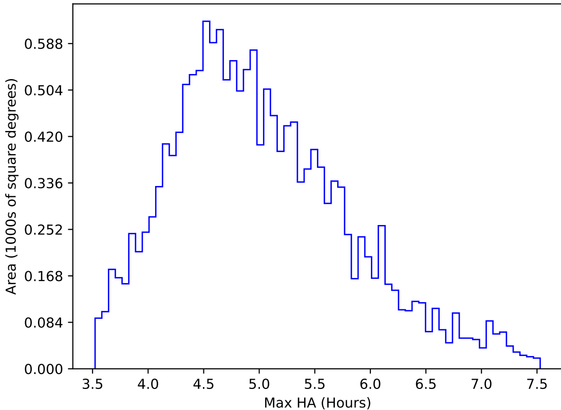
baseline_v3.0_10yrs WFD all bands: Max HA
