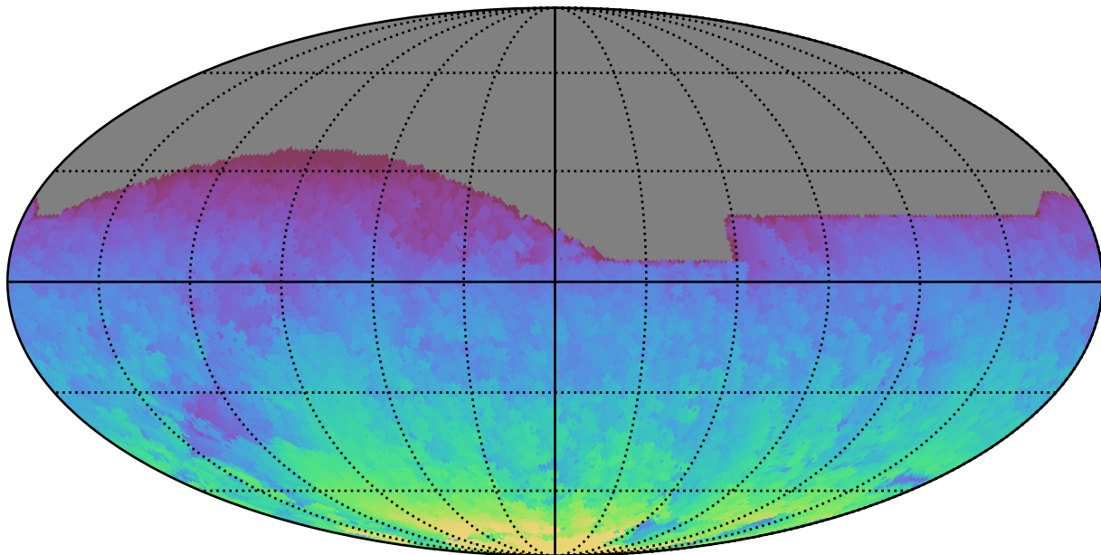
baseline_v3.0_10yrs All sky all bands: Max HA
