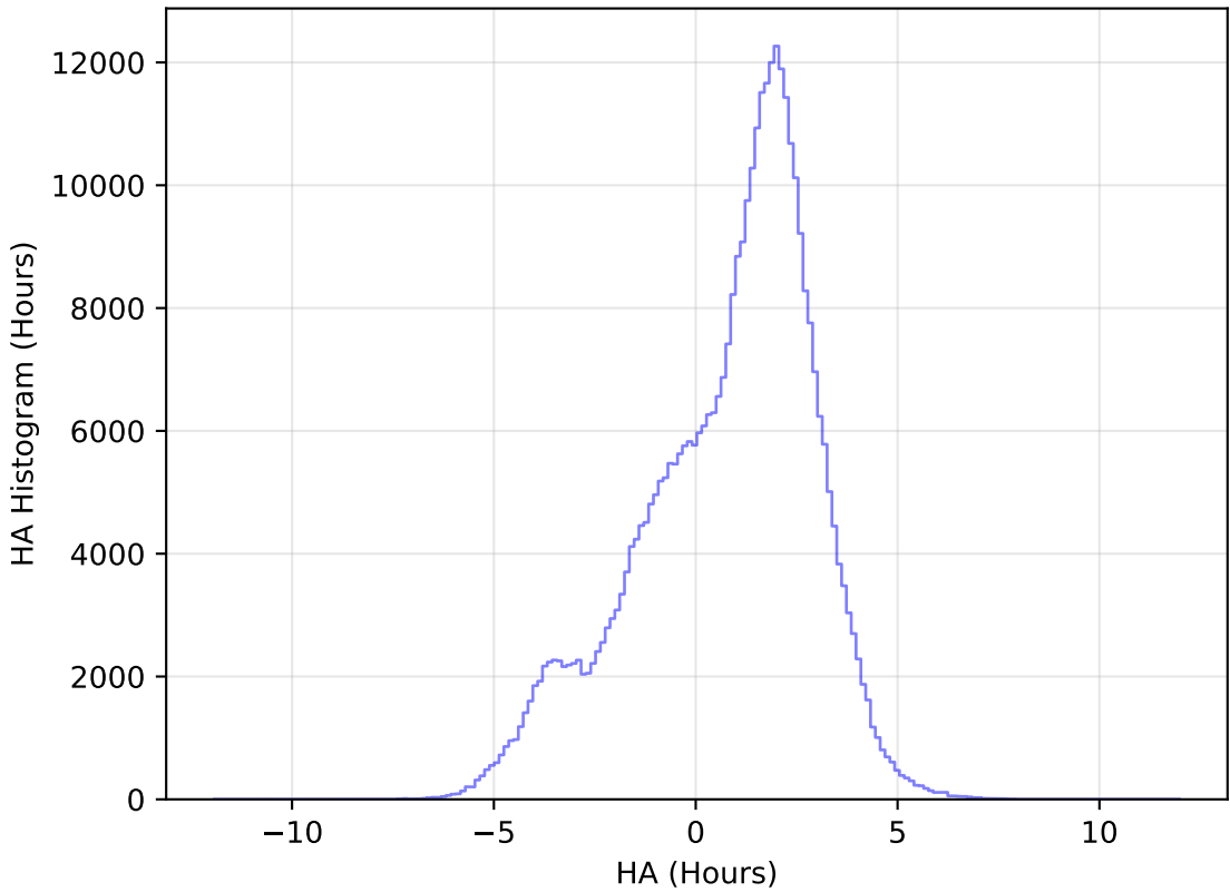
baseline_v3.0_10yrs WFD z band: HA Histogram
