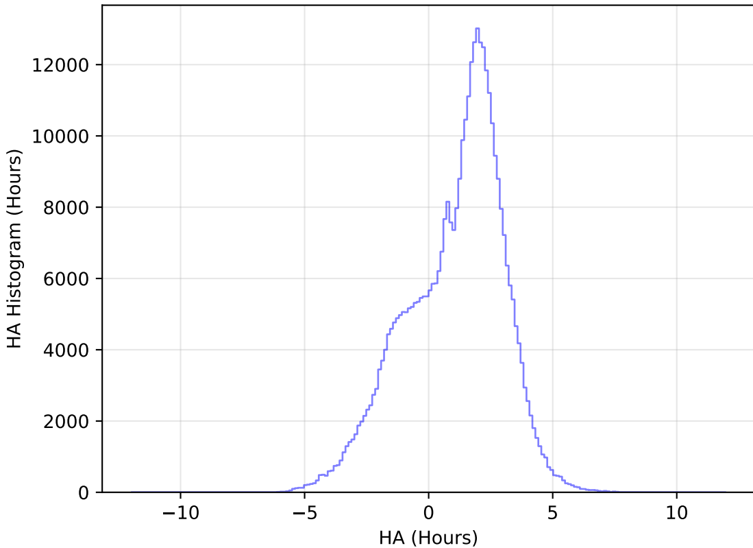
baseline_v3.0_10yrs WFD y band: HA Histogram
