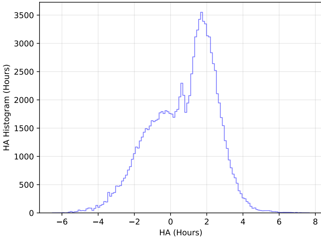
baseline_v3.0_10yrs WFD u band: HA Histogram
