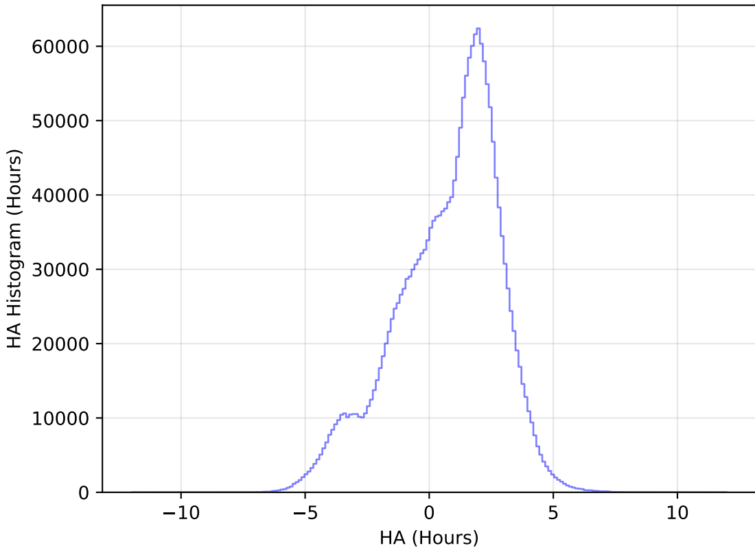
baseline_v3.0_10yrs WFD all bands: HA Histogram
