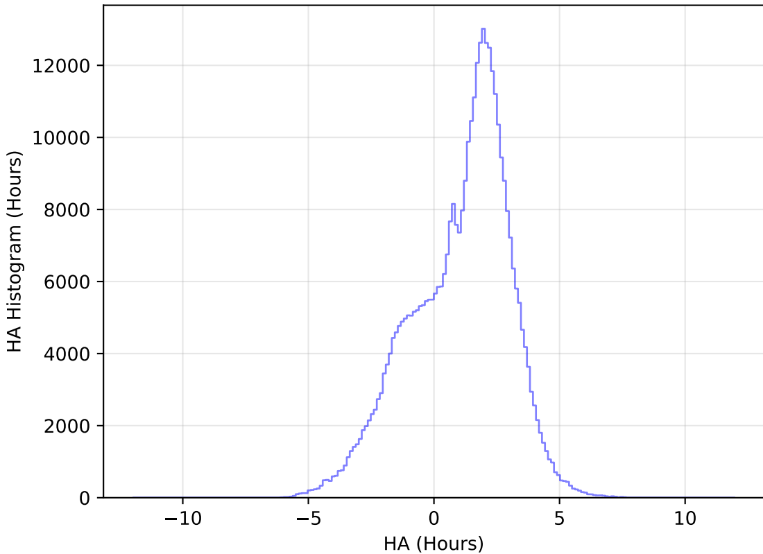
baseline_v3.0_10yrs All sky y band: HA Histogram
