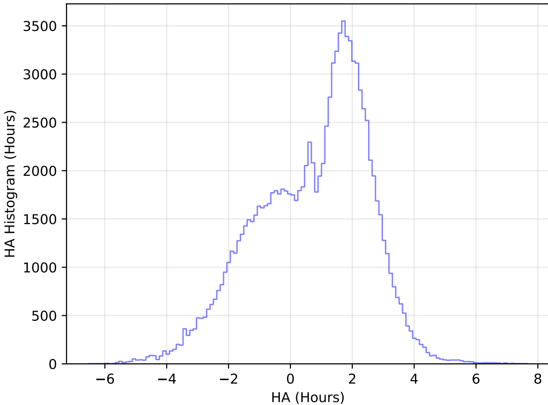
baseline_v3.0_10yrs All sky u band: HA Histogram
