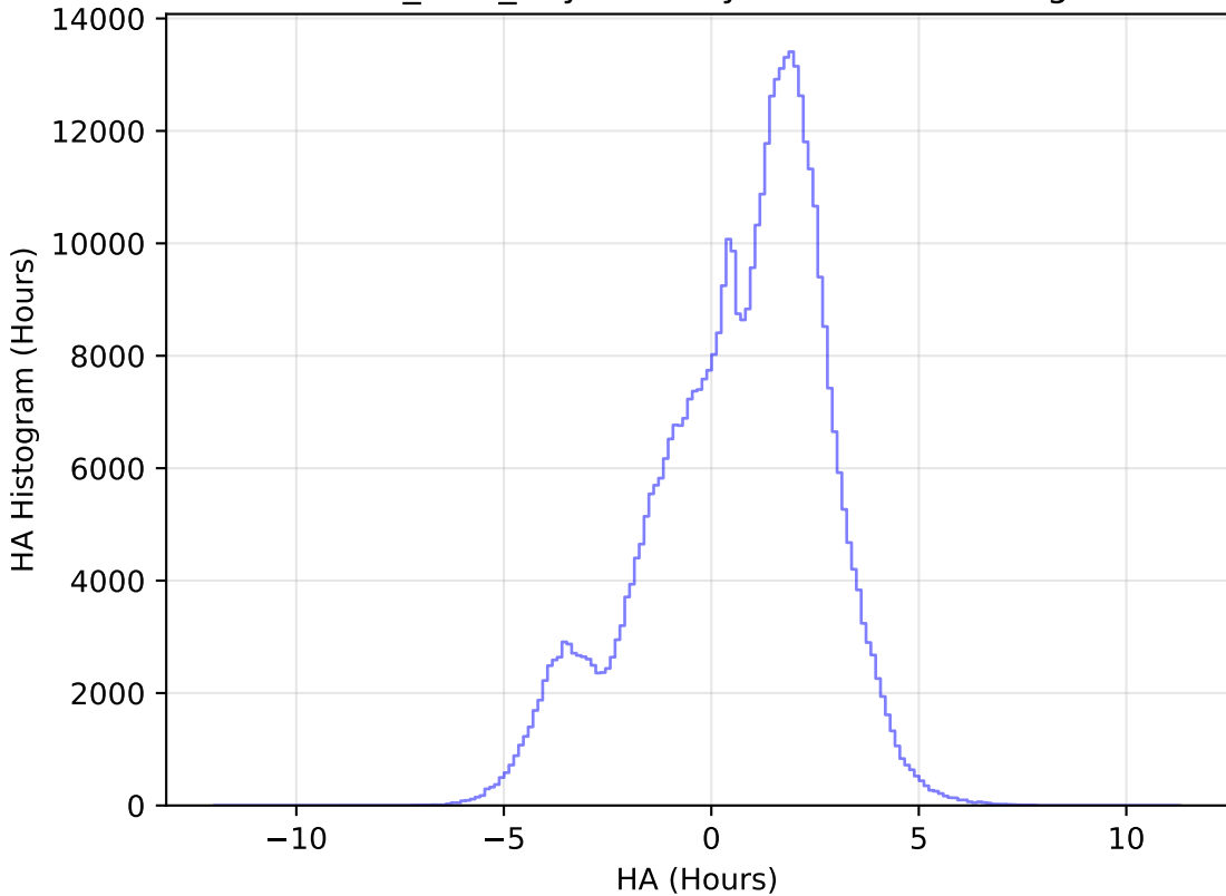
baseline_v3.0_10yrs All sky r band: HA Histogram
