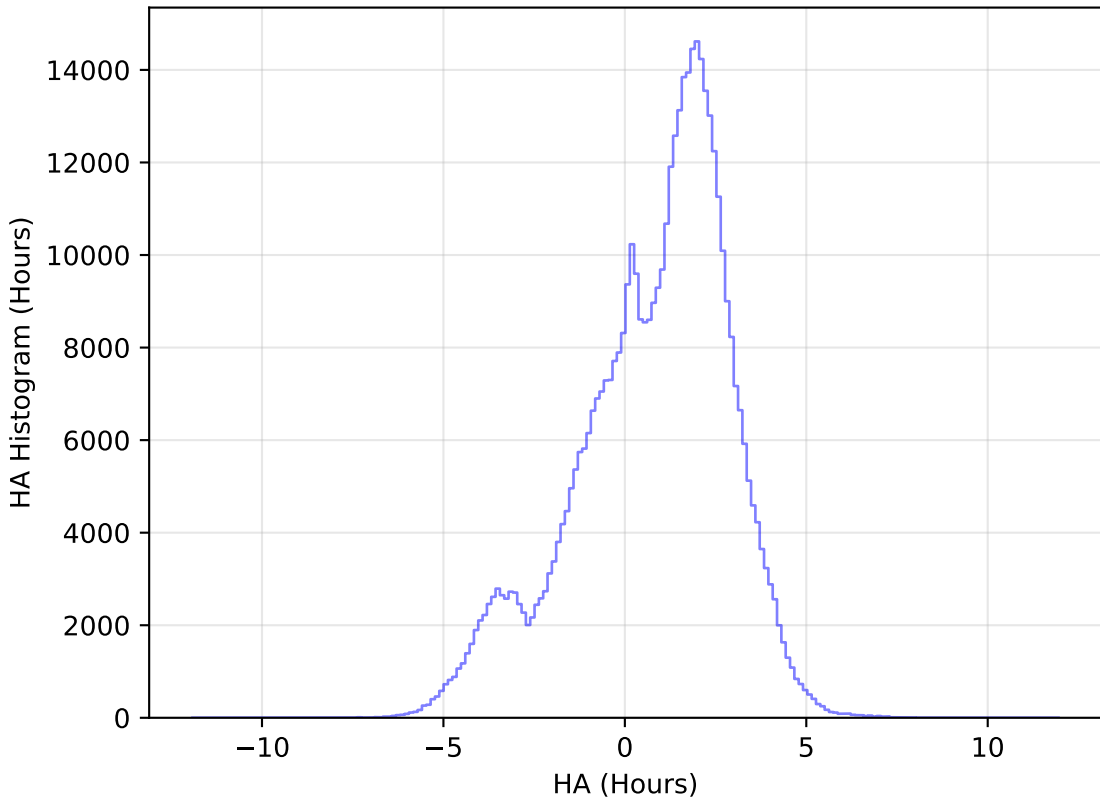
baseline_v3.0_10yrs All sky i band: HA Histogram
