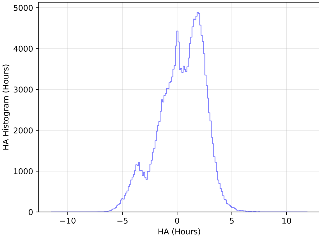
baseline_v3.0_10yrs All sky g band: HA Histogram
