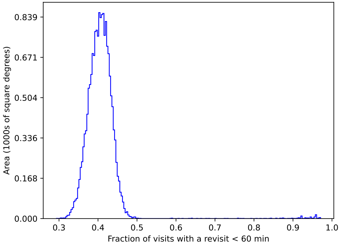
baseline_v3.0_10yrs gri WFD: Fraction of visits with a revisit < 60 min
