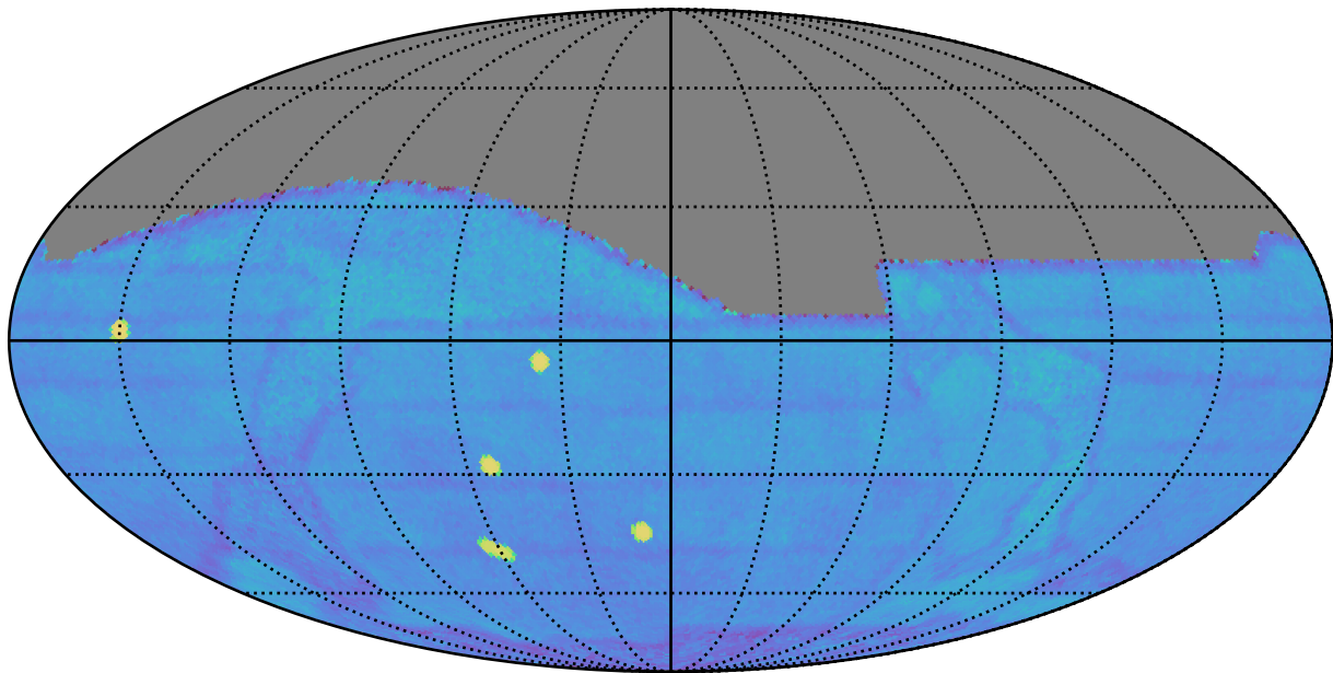
baseline_v3.0_10yrs gri All sky: Fraction of visits with a revisit < 60 min
