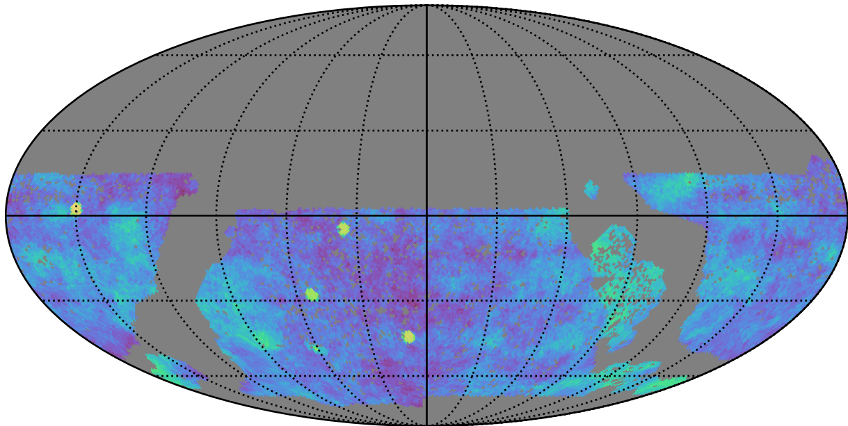
baseline_v3.0_10yrs gri WFD: Fraction of visits in pairs (20-90 min)
