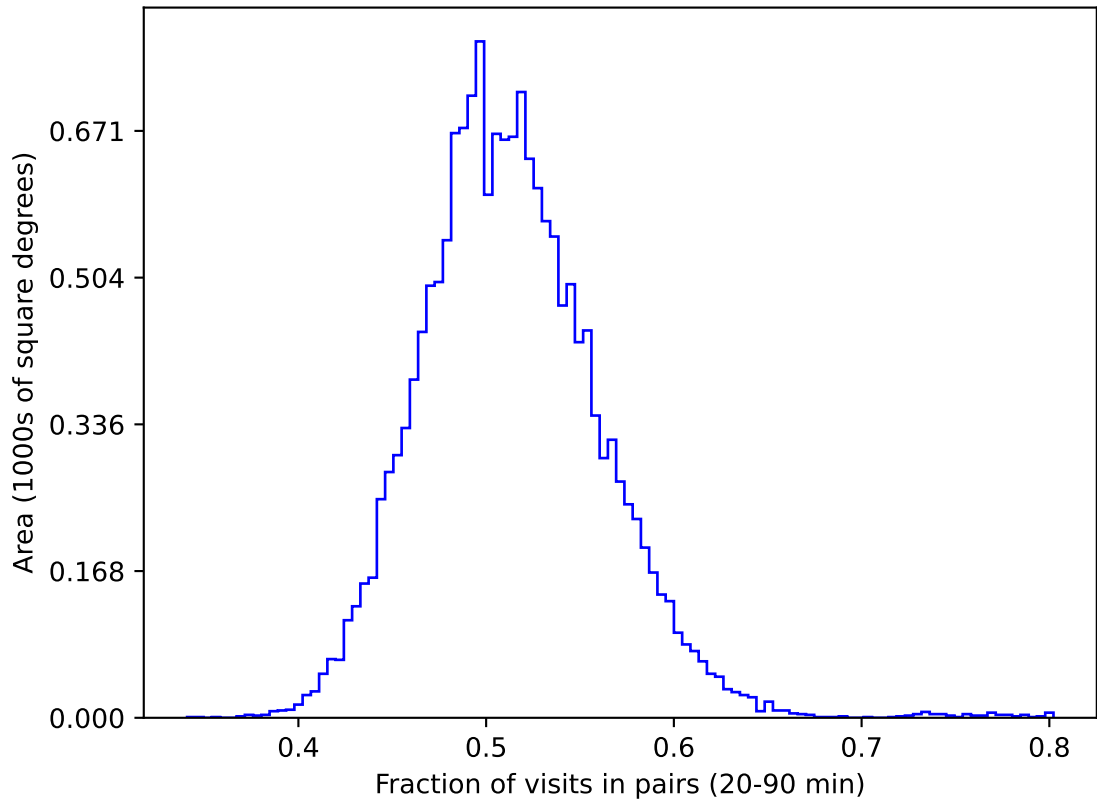
baseline_v3.0_10yrs gri WFD: Fraction of visits in pairs (20-90 min)
