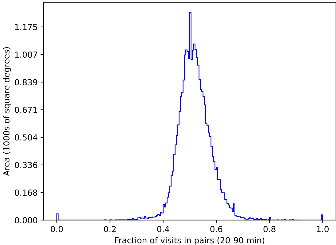
baseline_v3.0_10yrs gri All sky: Fraction of visits in pairs (20-90 min)
