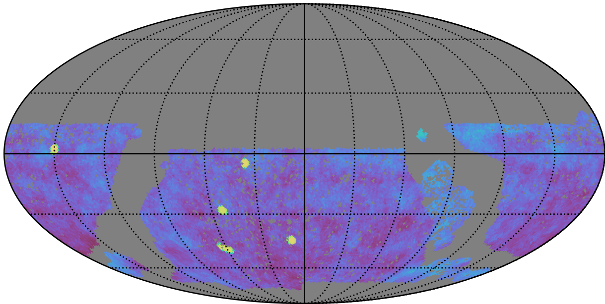
baseline_v3.0_10yrs gri WFD: Fraction of visits in pairs (10-60 min)
