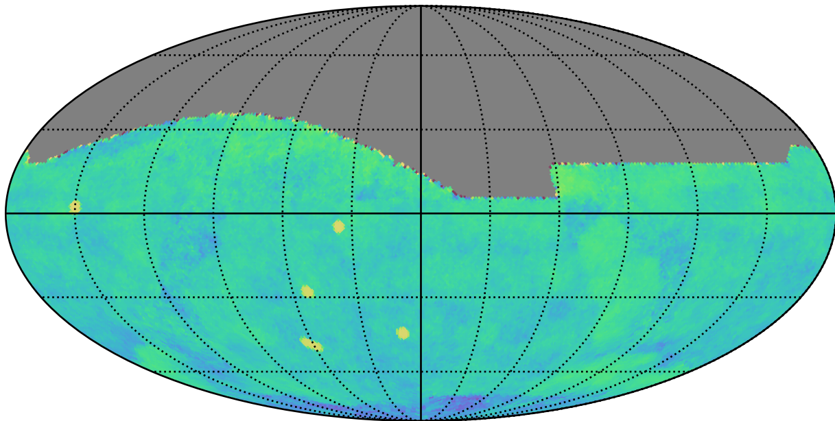
baseline_v3.0_10yrs gri All sky: Fraction of visits in pairs (10-60 min)
